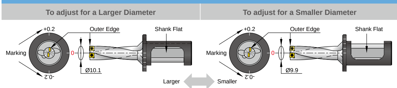
Fig. 1 Diameter Adjustment Method ( ex. Ø10 Drill )
